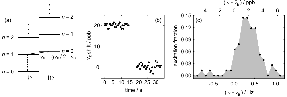
Figure 4.5: Anomaly quantum jump spectroscopy proceeds through discrete interrogations of the |0, \uparrow\rangle \leftrightarrow |1, \downarrow\rangle transition (a). A successful transition appears as a shift in the axial frequency when the |1\rangle state radiatively decays to the ground state (b). This frequency shift is a quantum nondemolition measurement. Multiple attempts at different frequencies may be binned into a histogram (c) to reveal the overall anomaly line.
