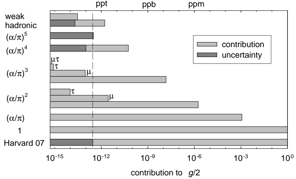
Figure 1.3: Theoretical contributions to the electron g
