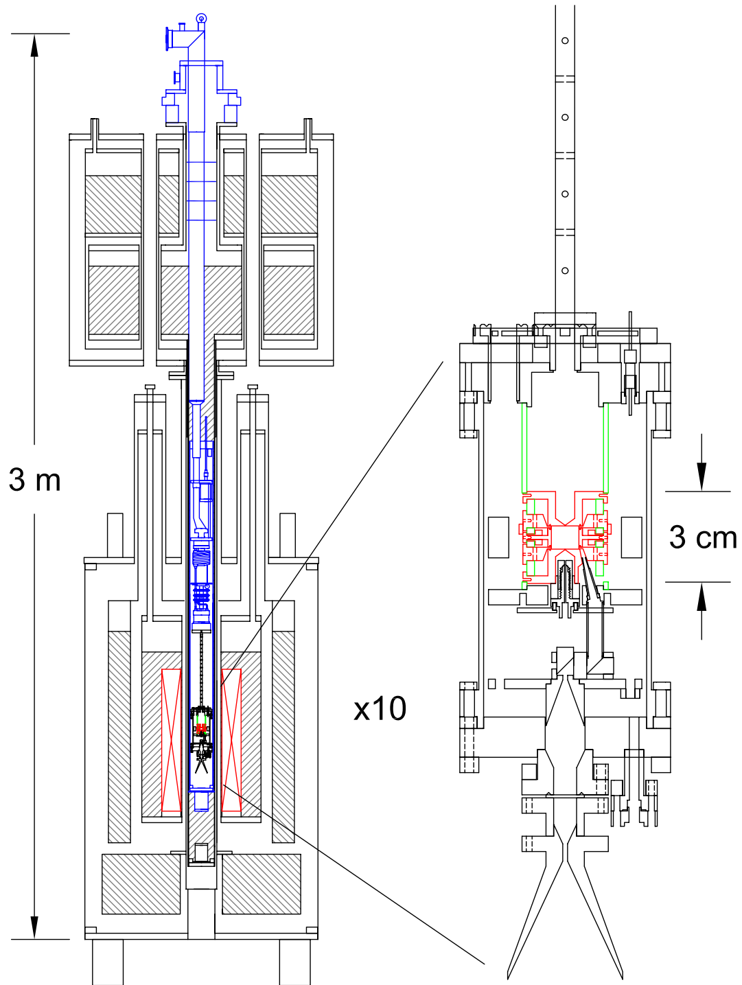
Figure 2.3: The entire apparatus
