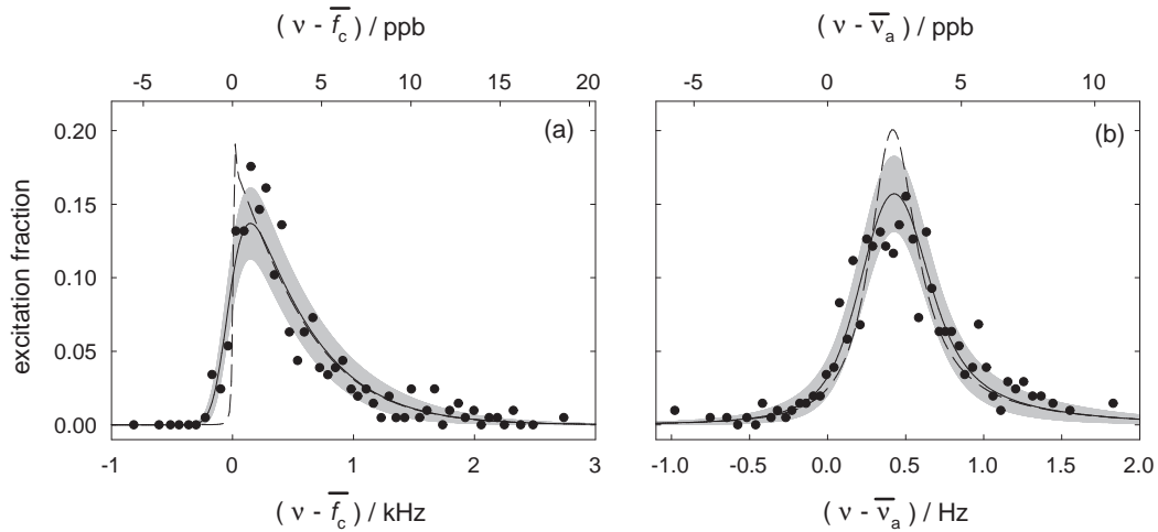
Figure 4.8: Results from maximum-likelihood fits to all of the 147.5 GHz cyclotron (a) and anomaly (b) data. To test the goodness of the fit, the individual attempt data have been binned into histograms (points). The gray bands indicate 68% confidence limits for distributions of measurements about the fit values. The dashed curves show the best-fit line with the Gaussian width set to zero.
